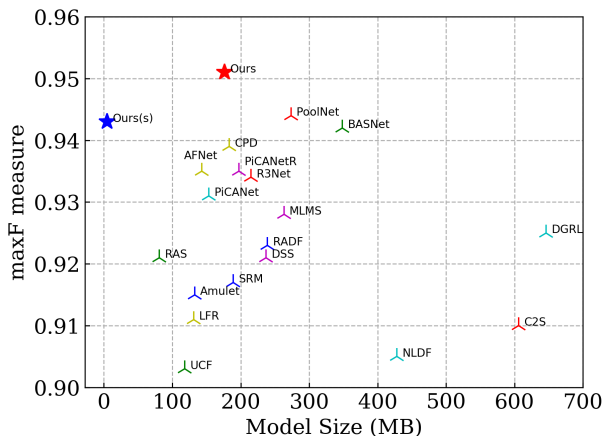
Figure 1. Comparison of model size and performance of our U 2 -Net with other state-of-the-art SOD models. The maxF_{\beta} measure is computed on dataset ECSSD [46]. The red star denotes our U 2 -Net (Ours) (176.3 MB) and the blue star denotes our small version U 2 -Net † (Ours † ) (4.7 MB).
